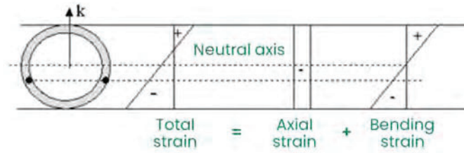
Figure 6: Total longitudinal strain distribution
