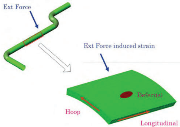
Figure 9 Schematic of loading conditions and strain consideration around a conventional defect
