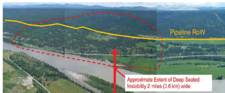
Figure 4b Landslide movement perpendicular to pipeline
