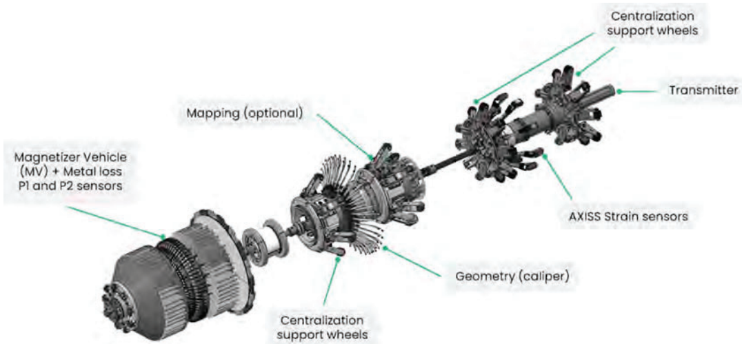
Figure 1: Standard configuration of ILI axial strain combo tool
