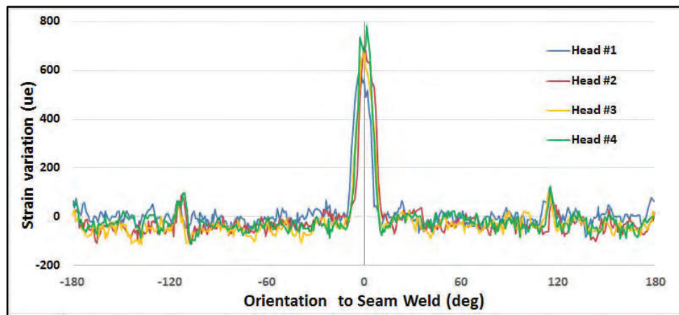
Figure 5: Average strain variation relative to seam weld orientation demonstrating the seam weld effect for 9.55mm WT X-52 grade for 30" pipe (circa 1957) [Ref 4-]
