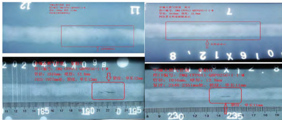
Figure 8: Example of cracks identified via threat assessment model vs original x-ray photos during construction
