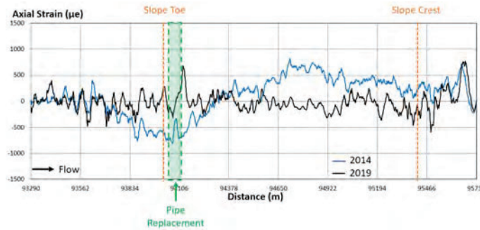
Figure 3: Axial strain profile on a pipeline for 2014 vs 2019 [ref 3-]
