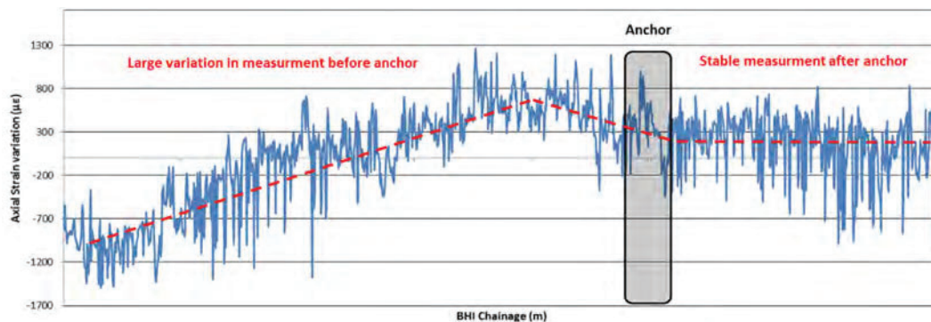
Figure 7: Axial strain trend illustrates ground movement stabilization after the anchor
