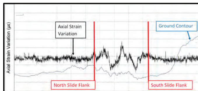
Figure 2: Defining the extent of a translational landslide on 13 km section of pipeline [ref 2]
