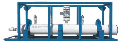
HYDROTEST HEADERS
